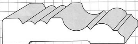
WM2012 3/4" x 3-1/2"
